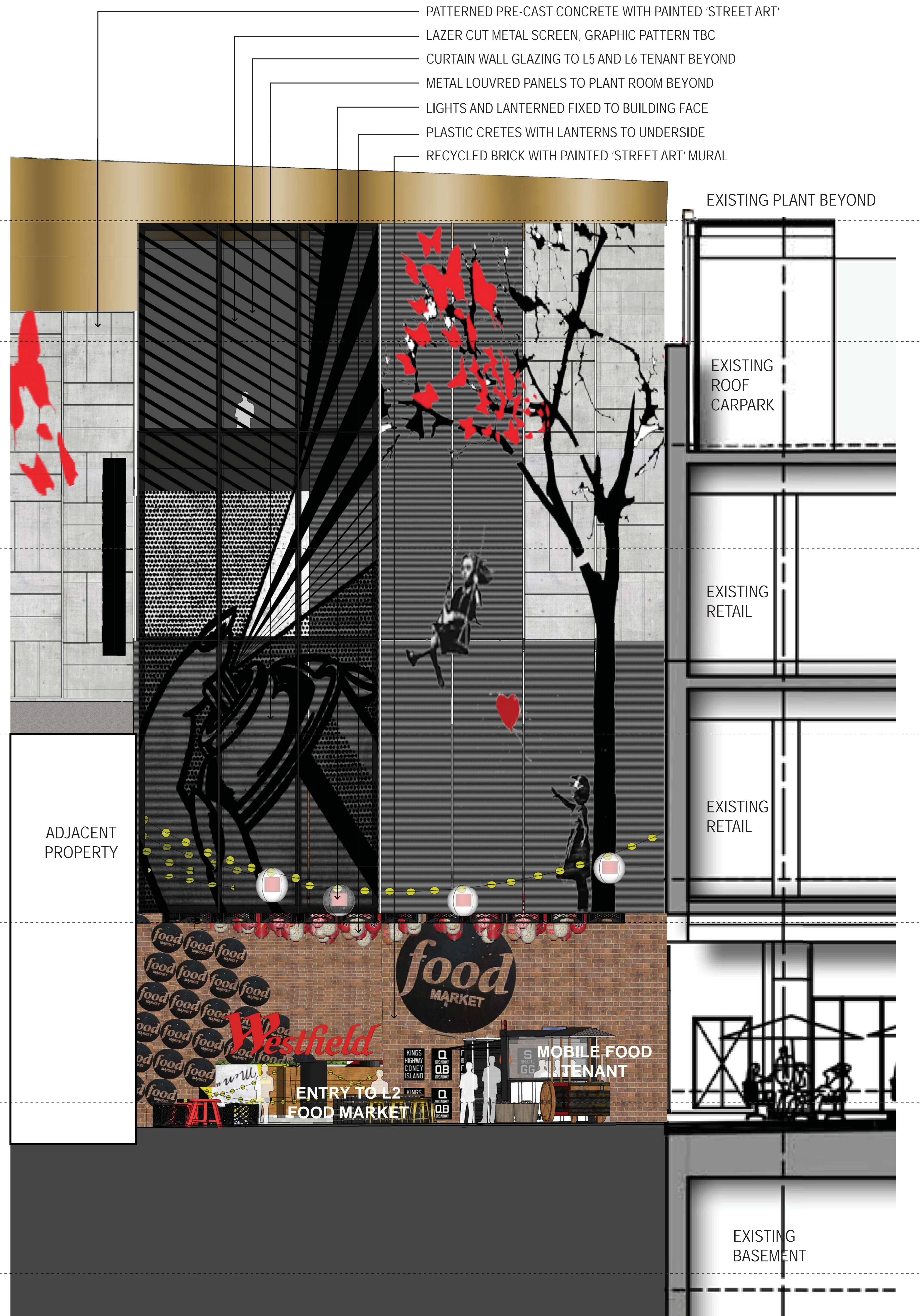
02 PROPOSED ELEVATION - CHARLOTTE LANE 1:50
