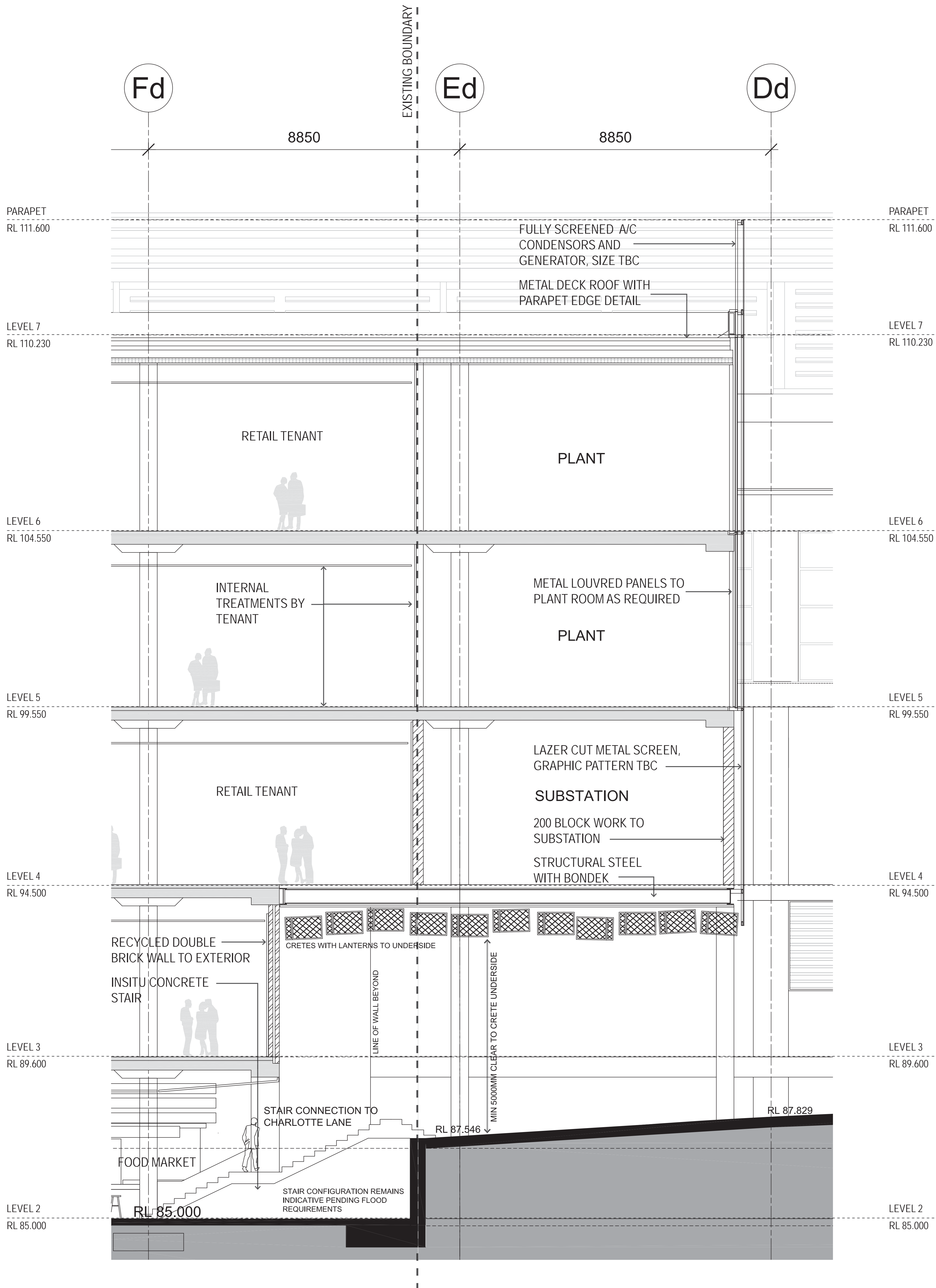
01 PROPOSED SECTION CHARLOTTE LANE CONNECTION 1:50
